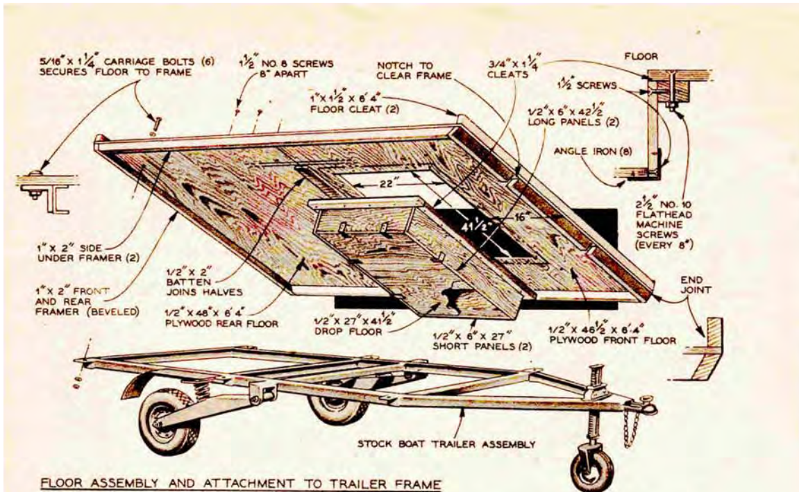
FLOOR ASSEMBLY AND ATTACHMENT TO TRAILER FRAME
